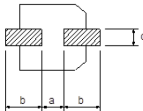
Fig. 5 Soldering pad
