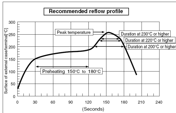
Figure 4 Reflow profile
