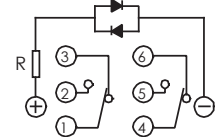
DPDT - DUAL COLOR LED
