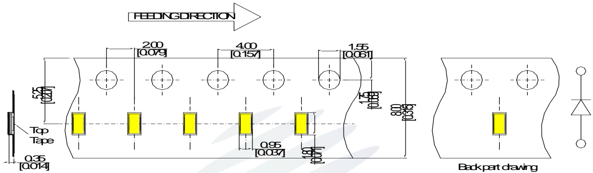
Fig.2-1 Carrier Tape Dimension 载带尺寸
