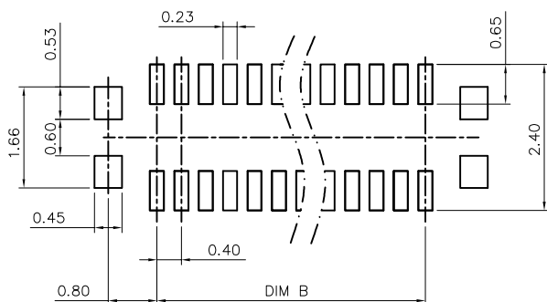
RECOMMENDED PCB LAYOUT(NO PATTERNS) ( TOLERANCE: ±0.02 )
