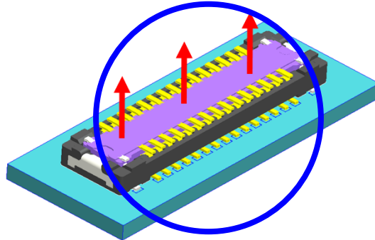
Releasing the plug paralleled to the mated axis 沿着组合轴向平行拔去
