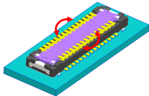
Releasing the plug by moving slowly in "b" direction 向左右一点点边晃动边拔去(短方向)
