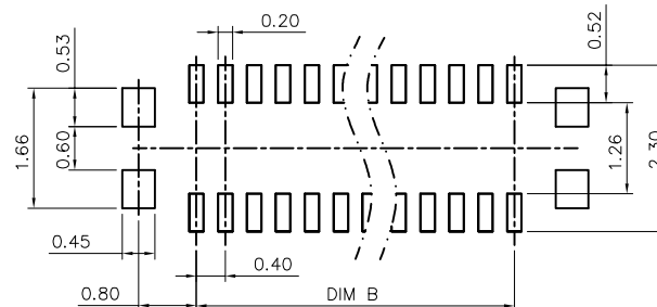
RECOMMENDED METAL MASK LAYOUT(NO PATTERNS) t=0.08mm ( TOLERANCE: ±0.01 )
