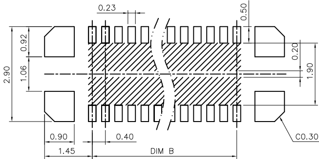
RECOMMENDED PCB LAYOUT(NO PATTERNS)
