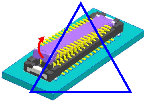
Slant releasing in "a" Direction (lengthways) 长方向的倾斜拔出
