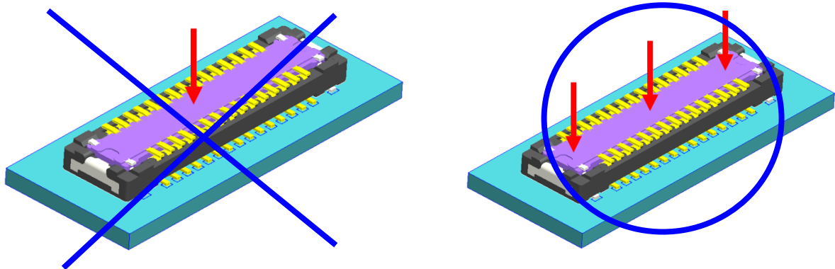
Pushing only Center(Wrong Handling) 只按压连接器中间部
