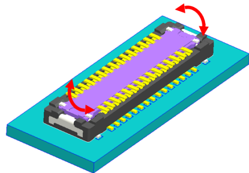
Releasing the plug by moving slowly in "a" direction (lengthways) 向左右一点点边晃动边拔去 (长方向)
