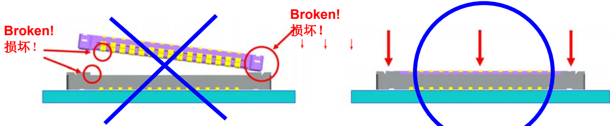
Mating with angle(Wrong Handling) 连接器倾斜组合
