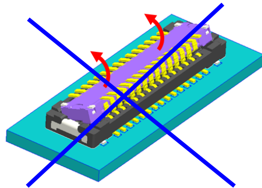
Slant releasing in "b" Direction 短方向的倾斜拔出
