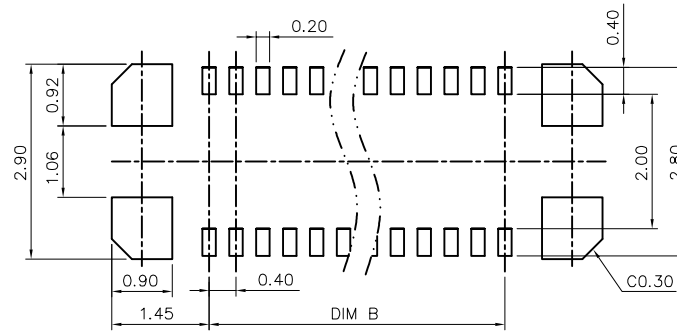
RECOMMENDED METAL MASK LAYOUT(NO PATTERNS) T=0.08mm
