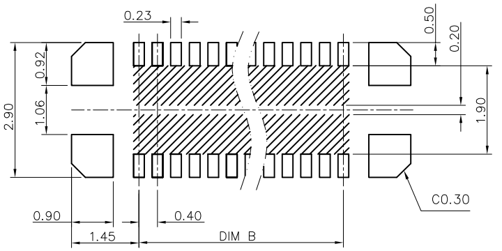
RECOMMENDED PCB LAYOUT(NO PATTERNS) ( TOLERANCE: ±0.03 )
