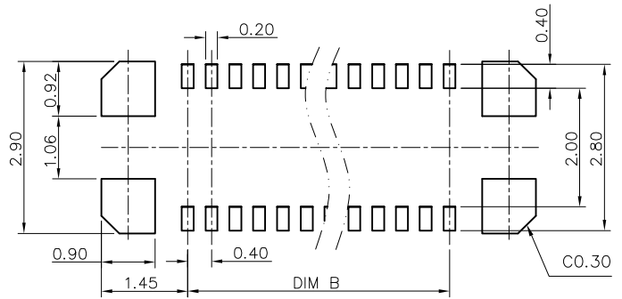
RECOMMENDED METAL MASK LAYOUT(NO PATTERNS) t=0.08mm ( TOLERANCE: ±0.01 )
