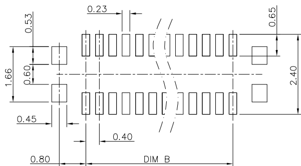
RECOMMENDED PCB LAYOUT(NO PATTERNS) ( TOLERANCE: ±0.03 )
