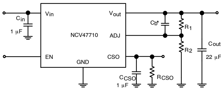
*Required if usage of low ESR output capacitor C_{out} is demand, see Regulator Stability Considerations section.
