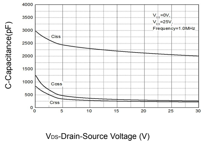
Figure 9: Capacitance Characteristics
