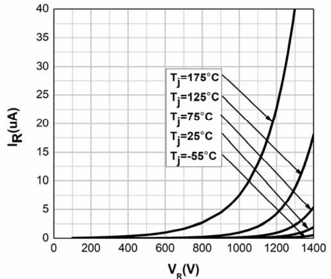
Figure2. Reverse Characteristic
