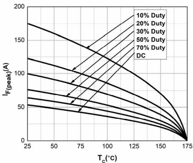
Figure 7. Current Derating
