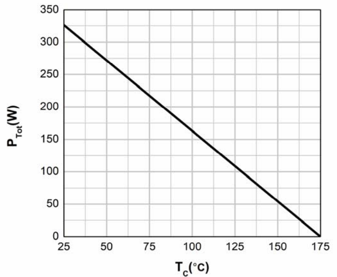
Figure 6. Power Derating
