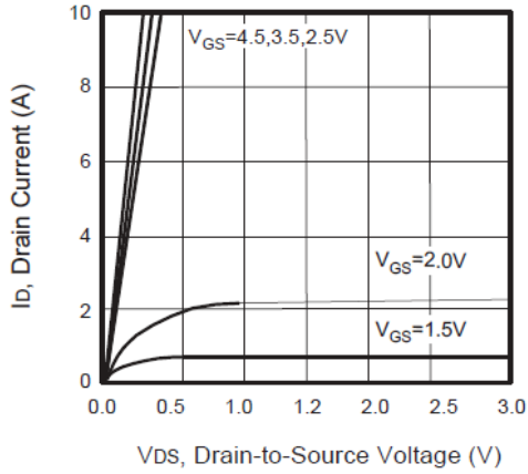
Figure 1. Output Characteristics
