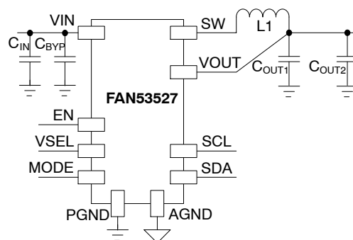
Figure 1. Typical Application
