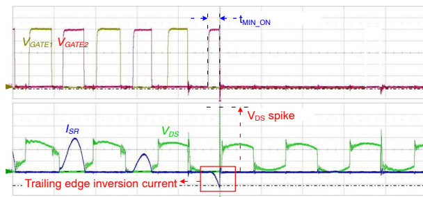
Figure 53. Trailing Edge Inversion Current
