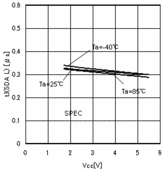
Figure 27. Noise removal time t_I (SDA L)
