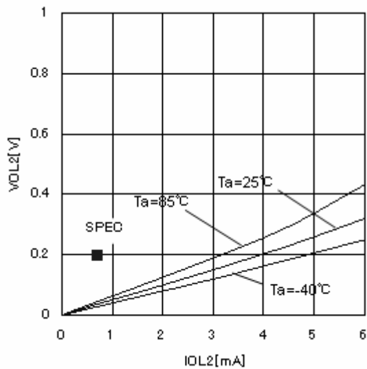
Figure 4. L output voltage V_{OL2-IOL2} ( V_{CC}=1.7V )
