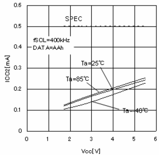
Figure 9. Consumption current at write action Icc2 (fSCL=400kHz)
