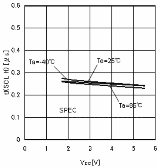
Figure 24. Noise removal time tI (SCL H)
