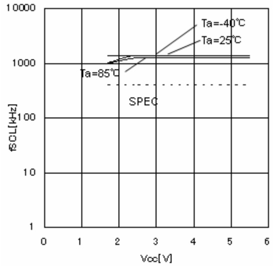
Figure 11. SCL frequency f_{SCL}
