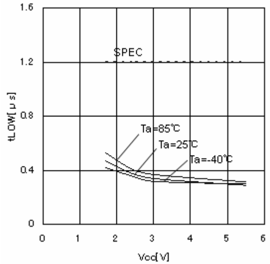
Figure 13. Data clock "L" time t_{LOW}
