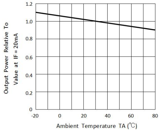
Fig.4 RELATIVE LUNIOUS INTENSITY VS. AMBIENT TEMPERATURE
