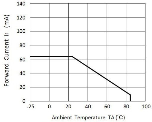
Fig.2 FORWARD CURRENT VS. DERATING CURVE
