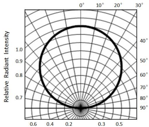
Fig6 RADIATION CHARACTERISTICS
