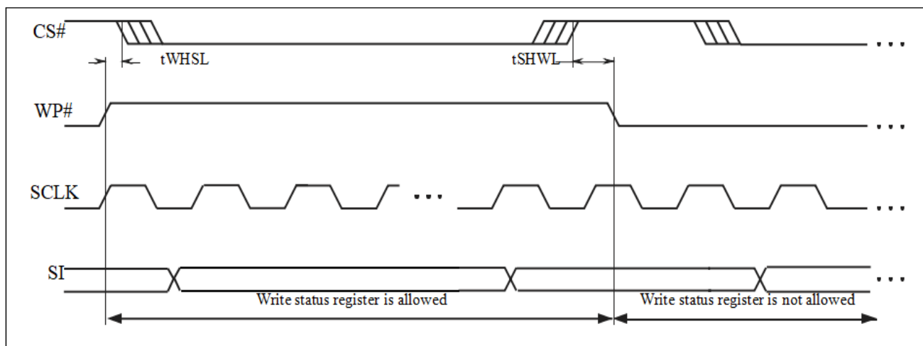
Figure 4-6 WP Timing
