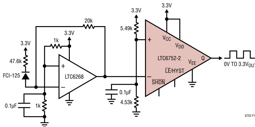
Figure 10. Optical Receiver Circuit
