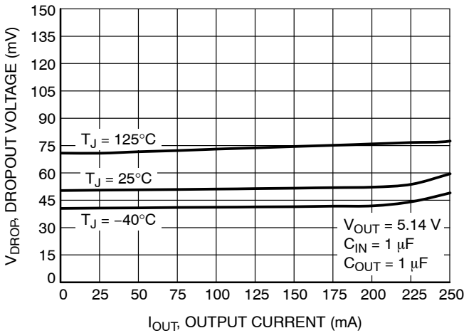
Figure 19. Dropout Voltage vs. Load Current - V_{OUT} = 5.14 V
