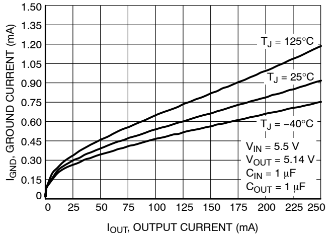
Figure 16. Ground Current vs. Load Current - V_{OUT} = 5.14 V
