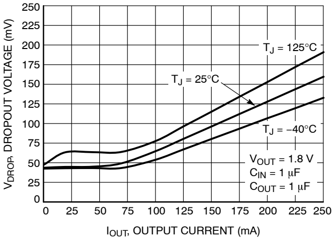
Figure 17. Dropout Voltage vs. Load Current - V_{OUT} = 1.8 V
