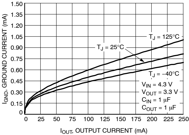
Figure 15. Ground Current vs. Load Current - V_{OUT} = 3.3 V
