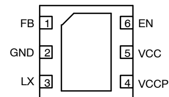
NCP1595A
