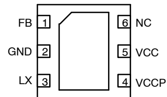
NCP1595/NCP1595C
