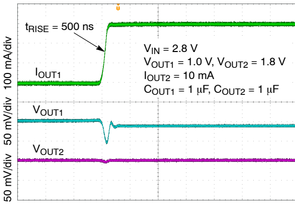
Figure 40. Load Transient Response – 1.0 V – Rising Edge, I_{OUT1} = 100\text{ μA} to 300 mA
