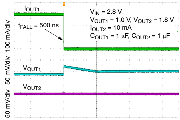
Figure 41. Load Transient Response – 1.0 V – Falling Edge, I_{OUT1} = 300\text{ mA} to 100 μA
