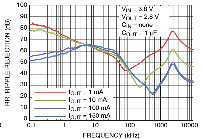
Figure 26. Power Supply Rejection Ratio, V_{OUT} = 2.8\text{ V} , C_{OUT} = 1\ \mu\text{F}
