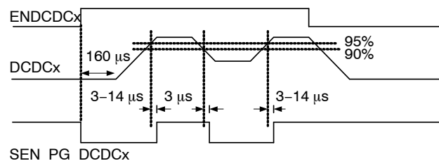
Figure 61. DCDCx Channel Internal Power Good Signal
