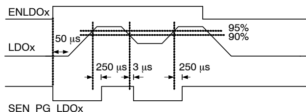
Figure 62. DCDCx Channel Internal Power Good Signal
