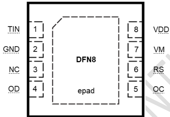
Figure 3 Pin Connection
