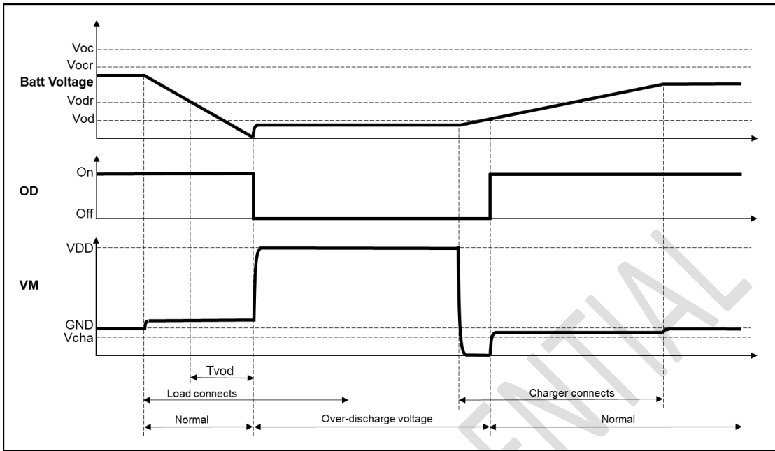
Figure 6 Charger Detection
