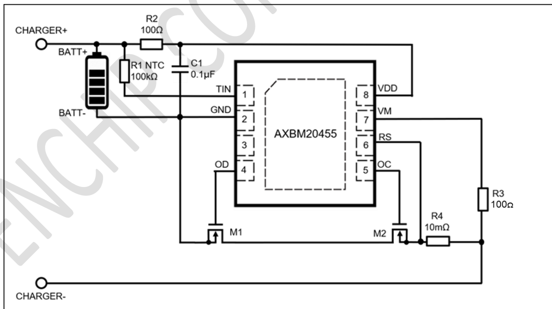
Figure 2 Application Circuit
