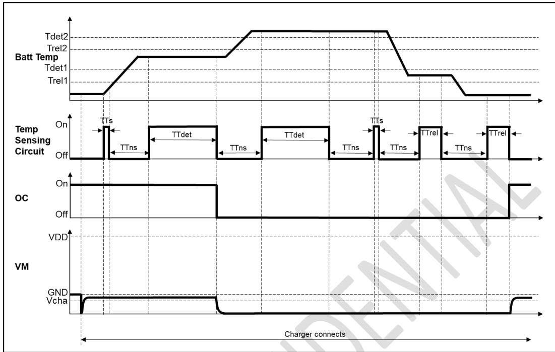
Figure 8 Thermal Detection (Charger Connects)
