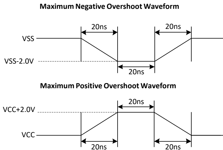
Figure38. Input Test Waveform and Measurement Level
