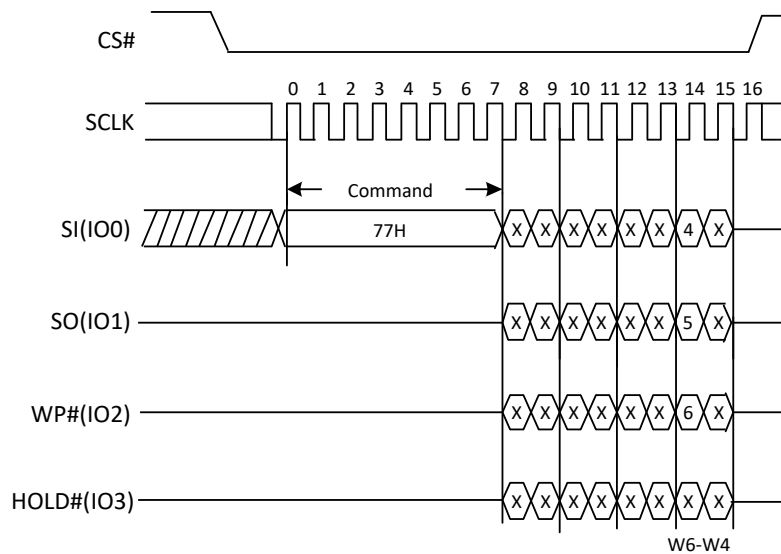
Figure 14. Set Burst with Wrap Sequence Diagram
