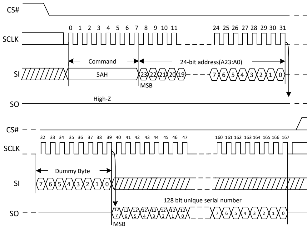
Figure 37.1. Read Unique ID (RUID) Sequence (Command 5AH)
