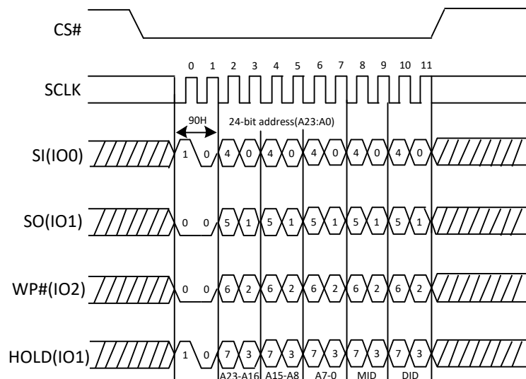
Figure 23a. Read Manufacturer ID/ Device ID Sequence Diagram (QPI)
