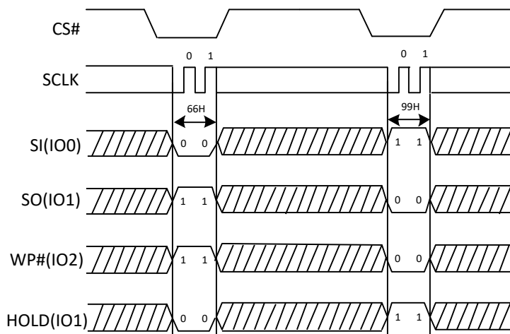
Figure 36a. Enable Reset and Reset command Sequence Diagram (QPI)
