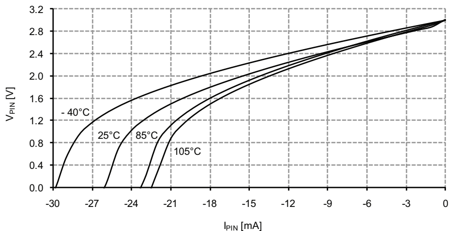
Figure 37-194. I/O pin output voltage vs. source current.
