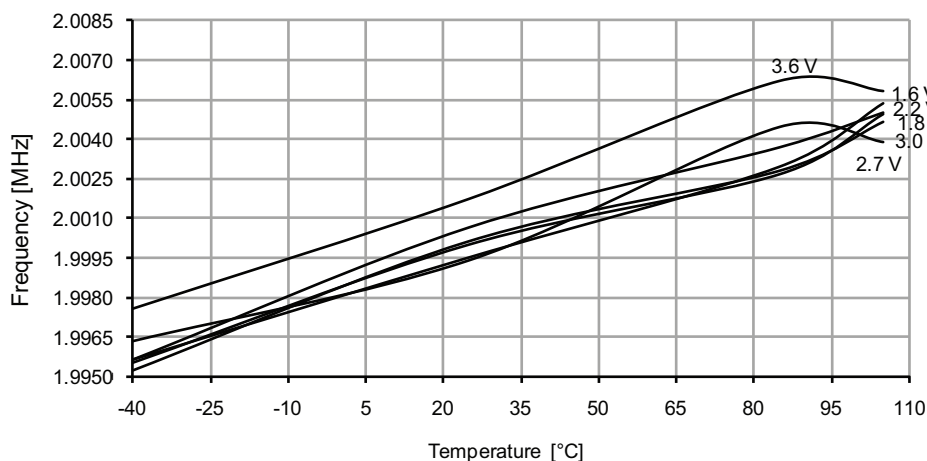
Figure 37-74. 2MHz internal oscillator frequency vs. temperature.
