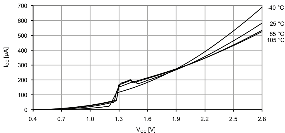
Figure 37-68. Power-on reset current consumption vs. V_{CC} .
