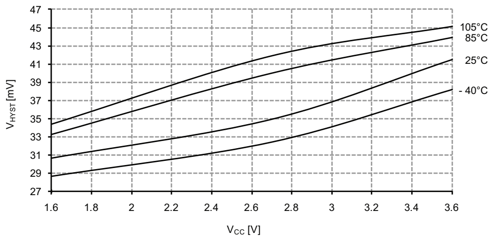
Figure 37-222. Analog comparator hysteresis vs. V_{CC} . High-speed mode, large hysteresis.
