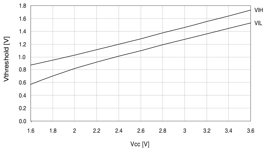
Figure 37-200. I/O pin input threshold voltage vs. V_{CC} .
