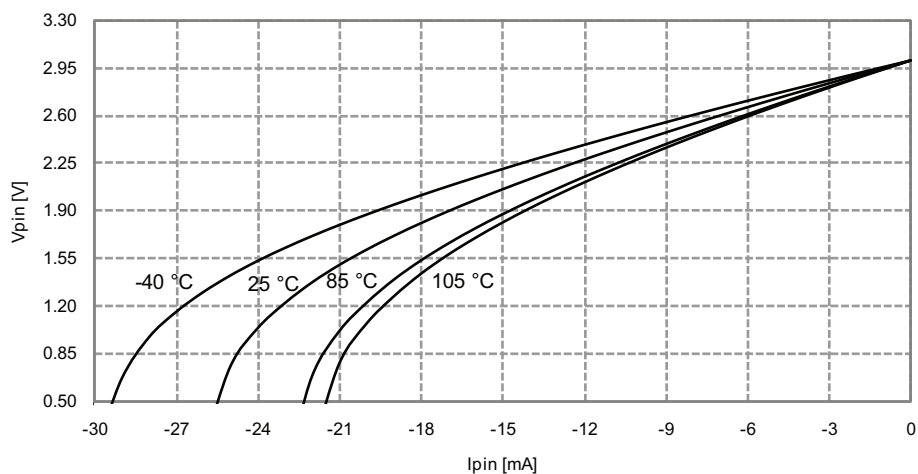
Figure 37-277. I/O pin output voltage vs. source current.
