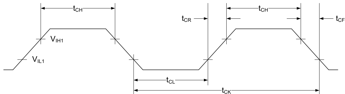
Figure 36-3. External clock drive waveform
