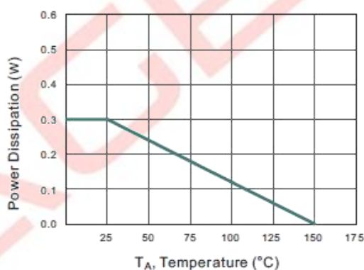
Fig.1 Maximum Continuous Power Derating
