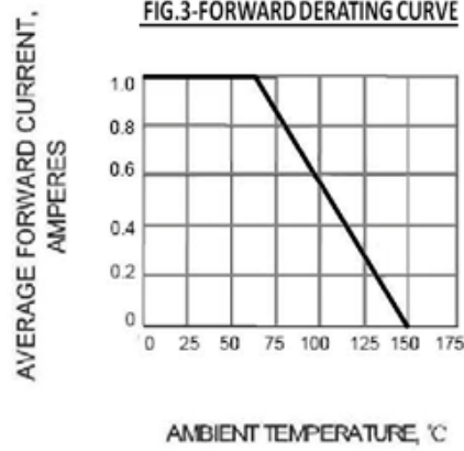
FIG.3-FORWARD DERATING CURVE
