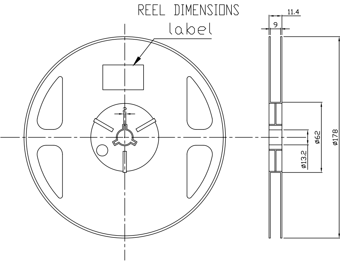
EMBOSSED TYPE DIMENSIONS
