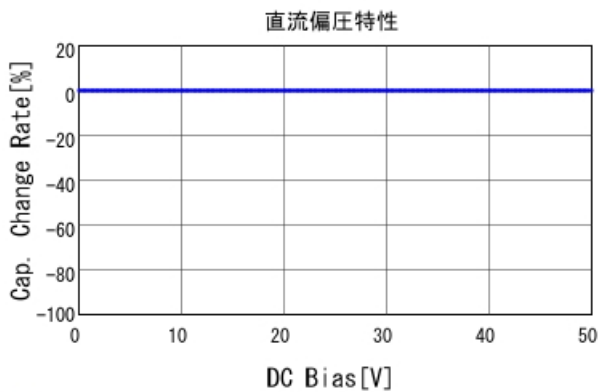
■ GCM1555G1H221JA16 C-DC bias capchange, 25.0degC, AC1V
