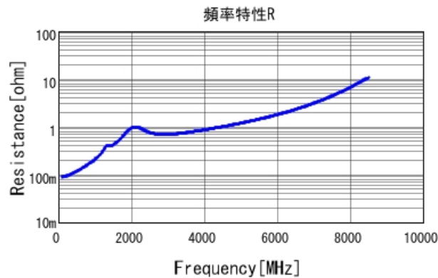
■ GCM1555G1H221JA16 R DC0V, 25degC
