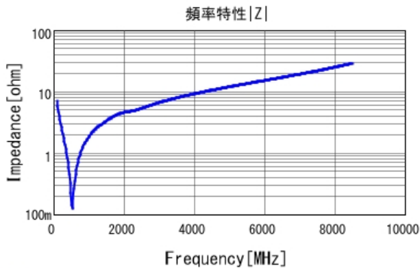
■ GCM1555G1H221JA16 |Z| DC0V, 25degC
