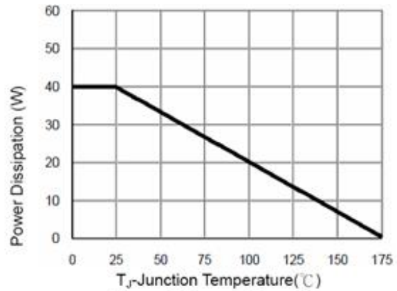
Figure 9 Power De-rating
