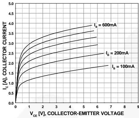
Figure 1. Static Characteristics
