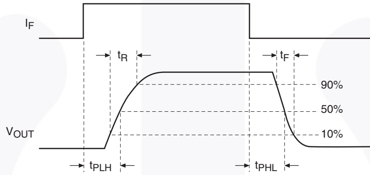
Figure 30. t_{PLH} , t_{PLH} , t_R and t_F Test Circuit and Waveforms
