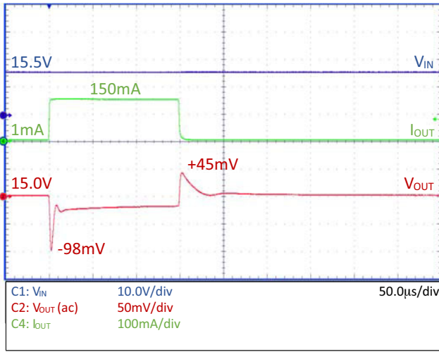
Figure 25. Load Transient – NCV8730–15.0 V, C_{OUT} = 22\text{ }\mu\text{F}
