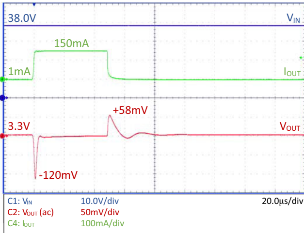
Figure 15. Load Transient – NCV8730–3.3 V, C_{OUT} = 1\text{ }\mu\text{F}
