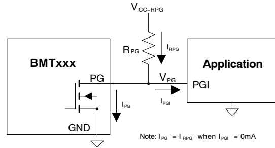
Figure 67. Circuit Example for R PG Value Selection
