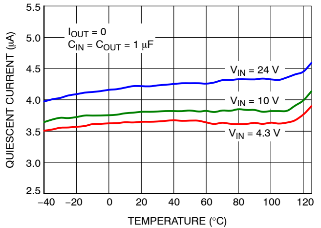
Figure 20. NCV8716x33xxx Quiescent Current vs. Temperature
