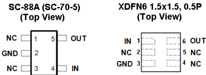
Figure 3. Pin Description
