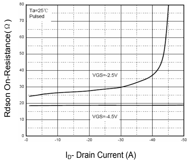
Figure 6 Drain-Source On-Resistance
