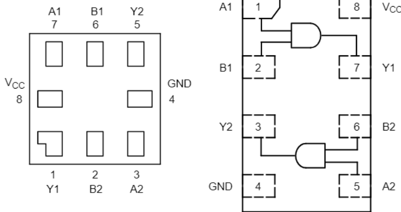
Figure 1. Pinouts
