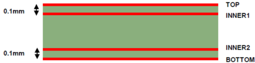
Figure 4. Recommended 4Layer PCB Options
