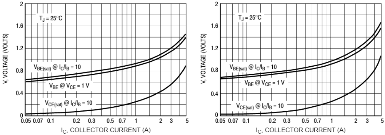
Figure 6. "On" Voltage
