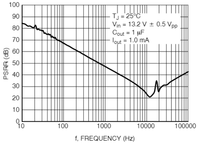
Figure 25. PSRR vs. Frequency (3.3 V Option)
