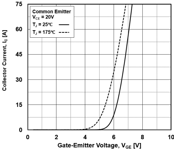
Figure 3. Transfer Characteristics
