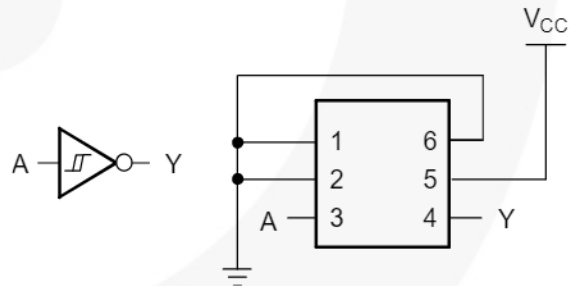
Figure 7. Inverter
