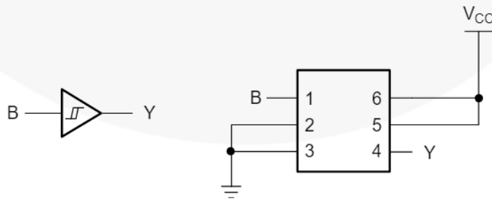
Figure 8. Non-Inverter Buffer
