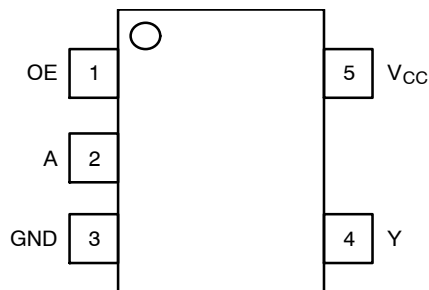
Pinout (126)
