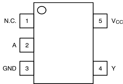
Pinout (Buffers and Inverters)
