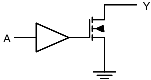
06 – Open-Drain Inverter
