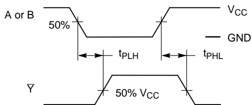
Figure 5. Switching Waveform
