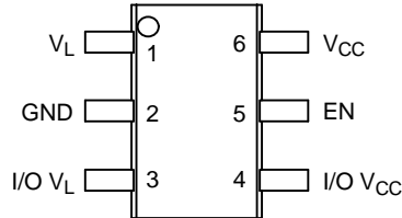
Figure 2. Pinout Diagram
