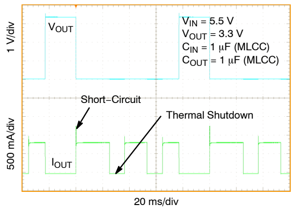
Figure 61. Short-Circuit and Thermal Shutdown
