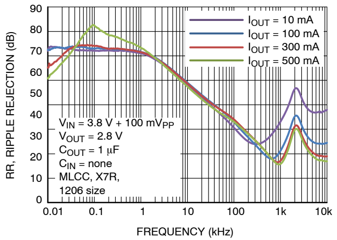
Figure 36. Power Supply Rejection Ratio, V_{OUT} = 2.8\text{ V}
