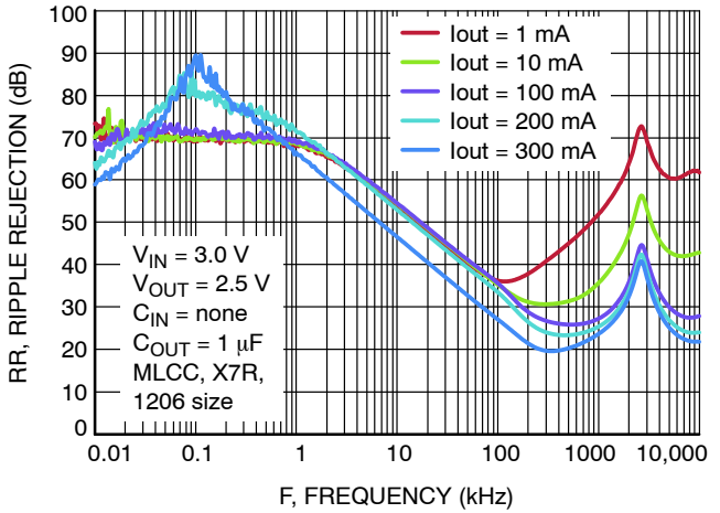
Figure 30. Power Supply Rejection Ratio, V_{OUT} = 2.5\text{ V}
