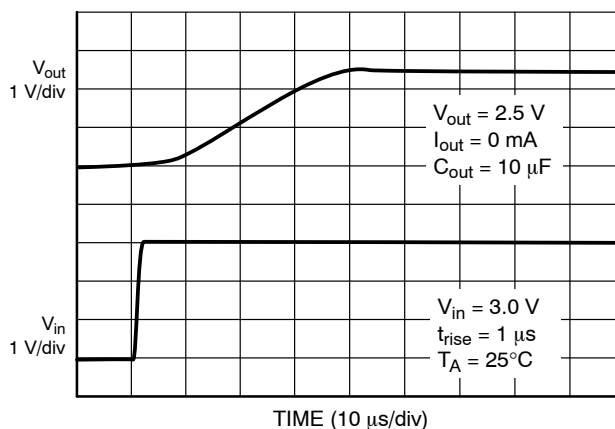
Figure 22. Startup Transient ( V_{out} = 2.5 V )
