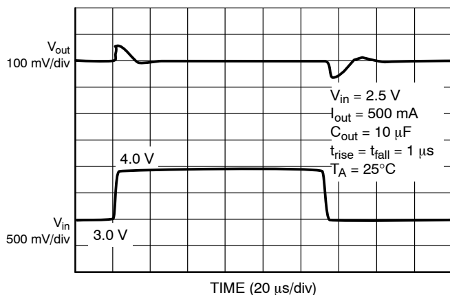
Figure 21. Line Transient ( V_{out} = 2.5 V )
